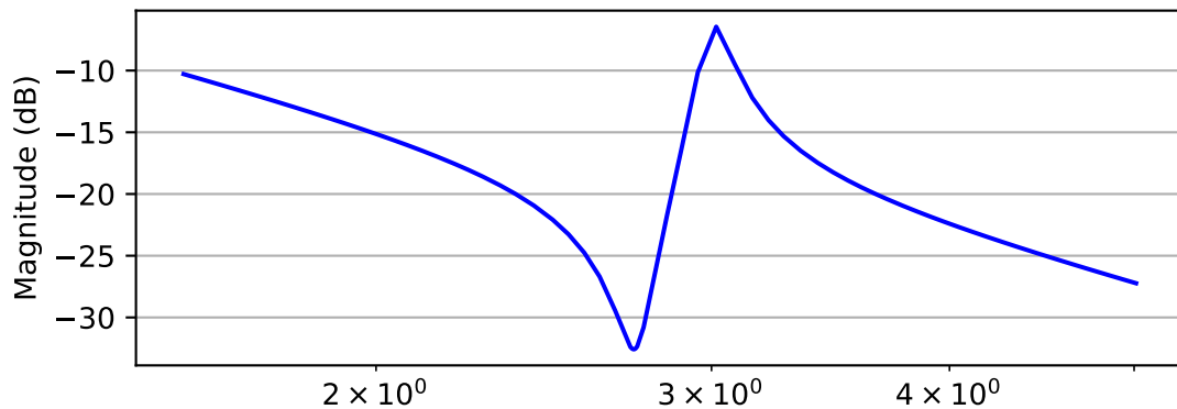
Bode Plot of \frac{s^2 + 0.1s + 7.5}{s^4 + 0.12s^3 + 9s^2}
